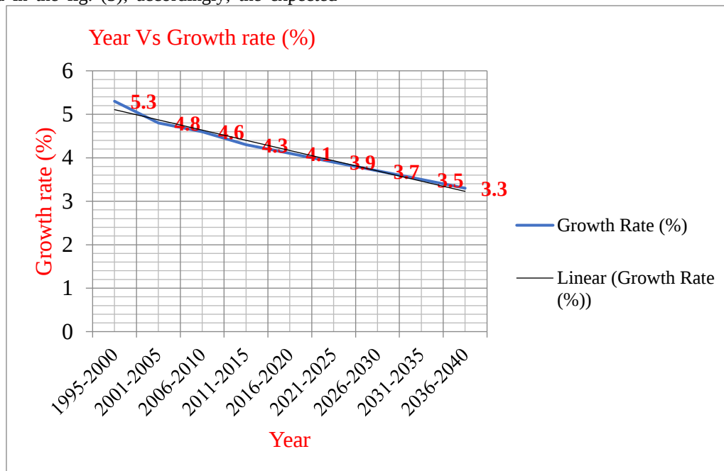
FIGURE 3: LINEAR EXTRAPOLATION OF ANNUAL GROWTH RATE
